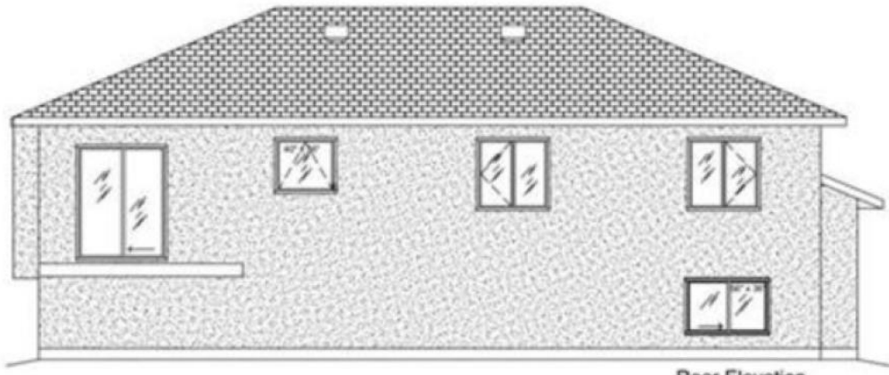
Rear Elevation SCALE: 3/16" = 1'-0"
